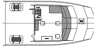
PILOT HOUSE PLAN
