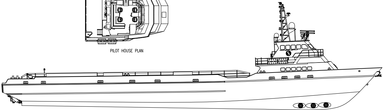
OUTBOARD PROFILE
