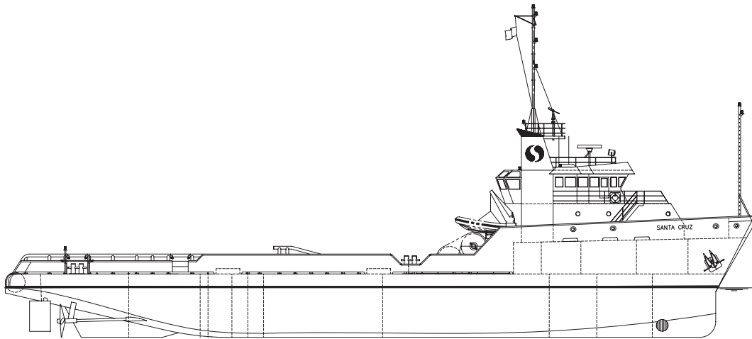
OUTBOARD PROFILE
