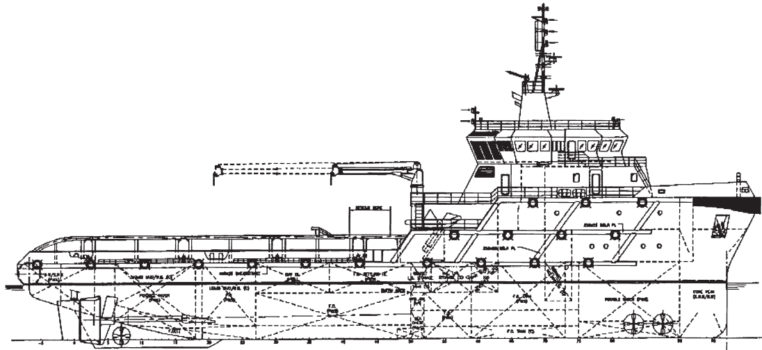
OUTBOARD PROFILE
