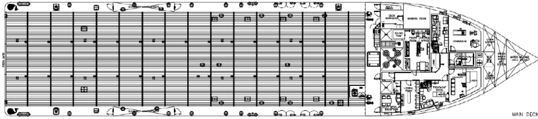
MAN DECK
